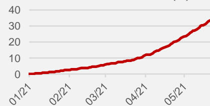
Share of people who received at least one dose of COVID-19 vaccine (%)
